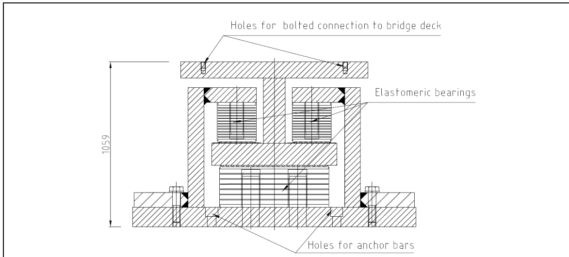
Fig. 2: Cross section (transverse) through bearing
