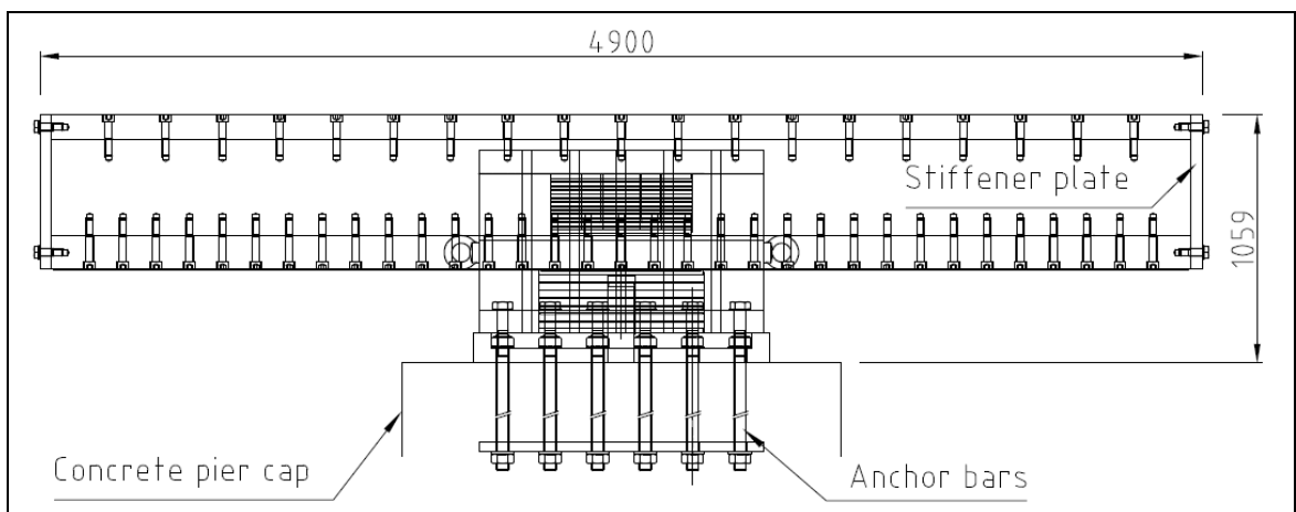
Fig. 3: Cross section (longitudinal) through bearing
