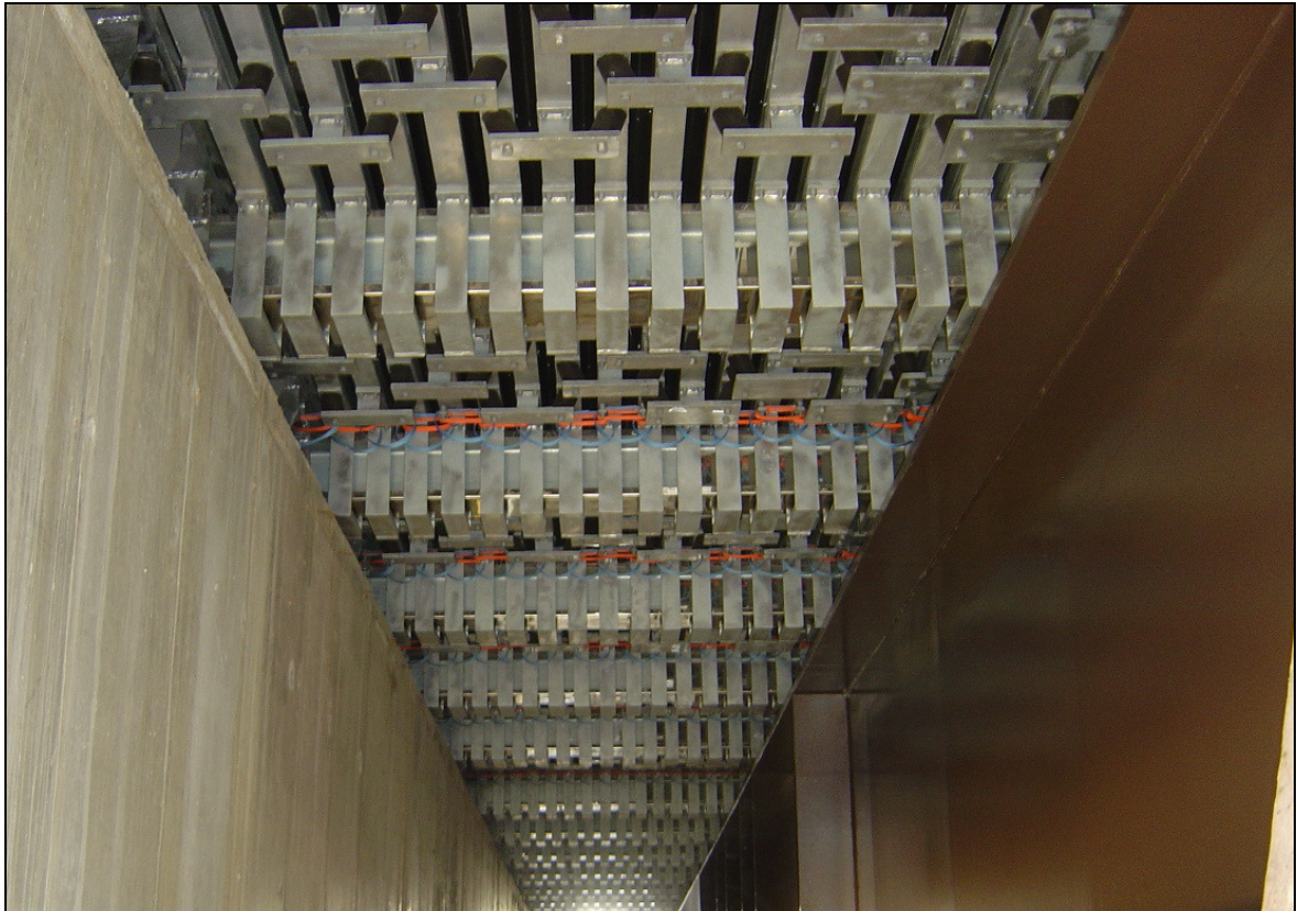
Fig. 11: A large modular expansion joint after installation, viewed from below
