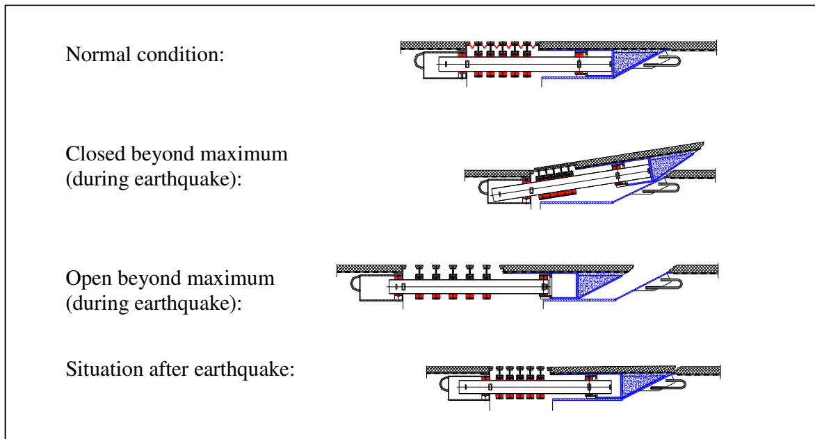
Fig. 8: Principle of the Fuse-Box system
