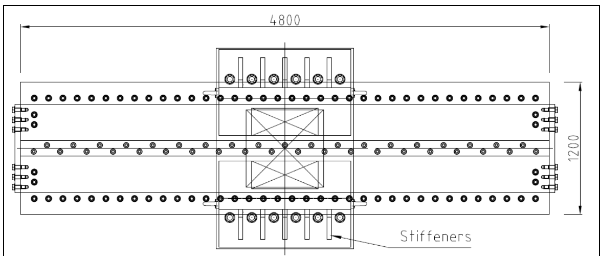
Fig. 4: Plan on bearing
