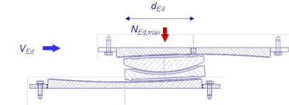
2 b) Seismic condition
